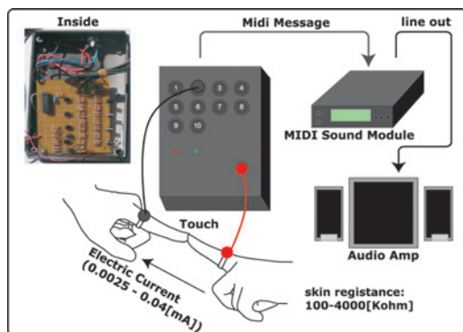
Figure 3: Overview of Freqtric Drums system.
