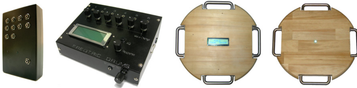
Figure 2: Prototypes of Freqtric Drums. FDL, FDL2, FDH and FDH2
